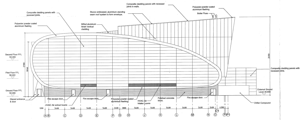
SOUTH ELEVATION
