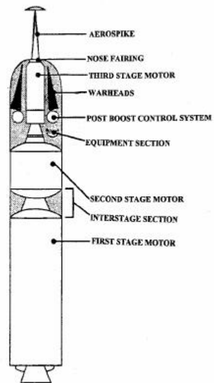
Trident-2 (D-5) Missile Source: US Navy
