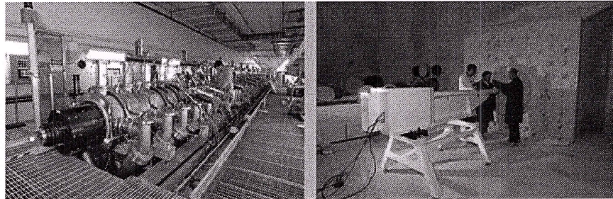
Mechanical technologist Keith Lewis works on the Flash X Ray (FXR) accelerator, an important diagnostic tool for hydrodynamic testing. The firing chamber is behind the wall at the far end of FXR.
