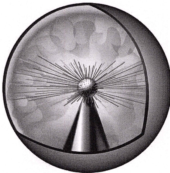
A cutaway of an experimental device shows a pin-dome diagnostic for evaluating the implosion of a device. As the sphere implodes, signals from the pins track the imploded material moving toward the center, thereby providing data about the temporal and spatial uniformity of the implosion.
