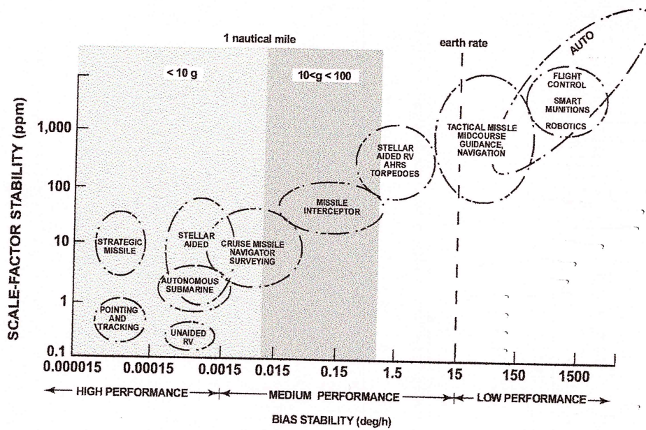
Figure 16.1-2. Gyroscope Technology Applications (shaded areas are militarily critical regions)
