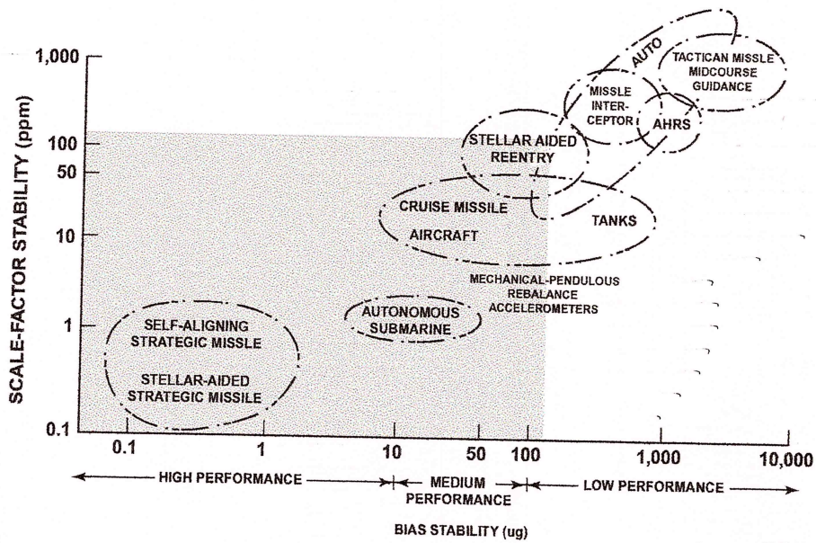
Figure 16.1-1. Accelerometer Technology Applications (shaded area is militarily critical region)
