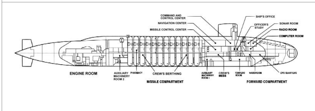
Figure 9: US Ohio-class SSBN showing missile compartment
